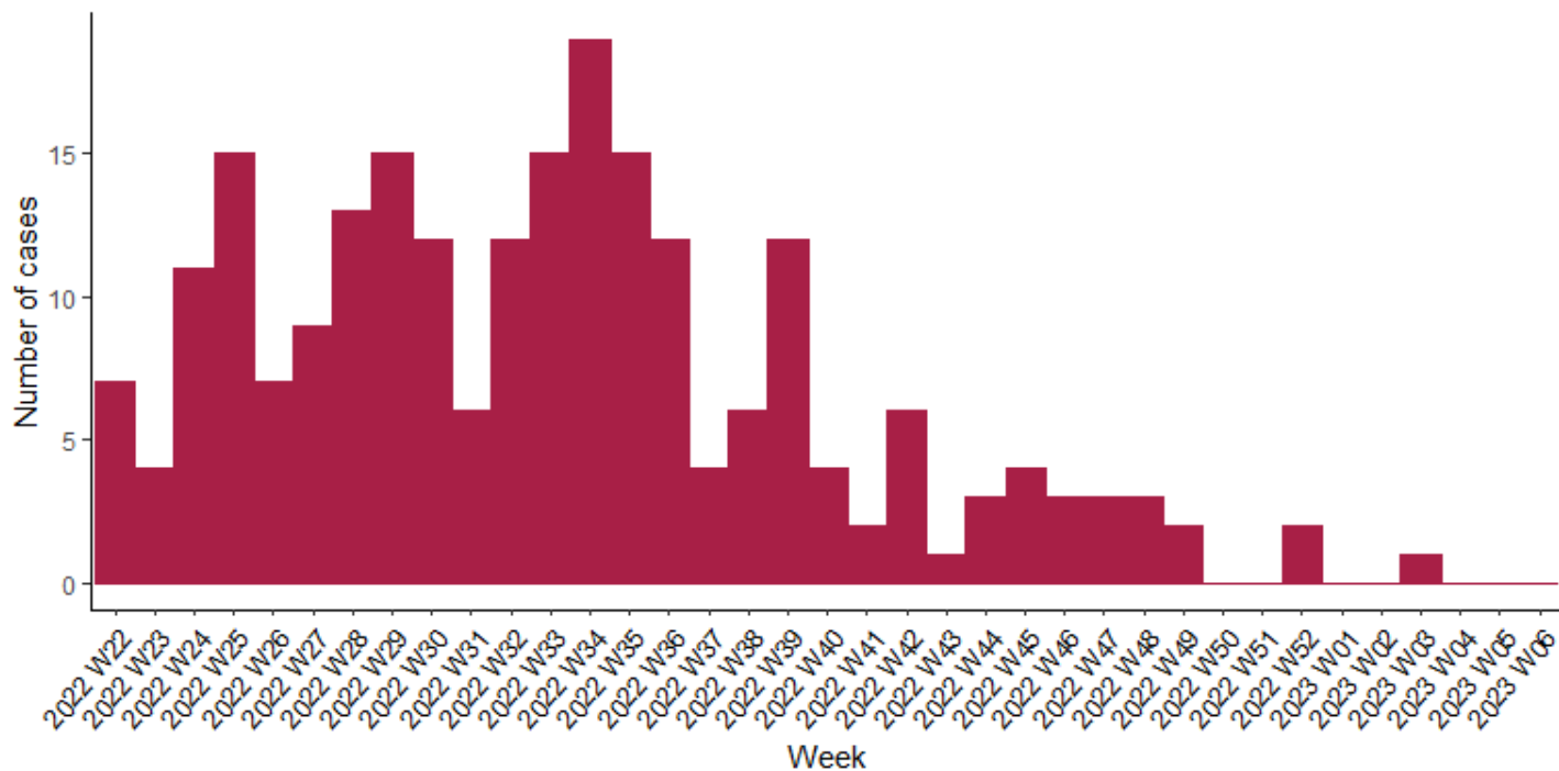
Figure 1: Number of confirmed cases of mpox by week of notification reported on CIDR in Ireland up to midnight 11-02-2023.
